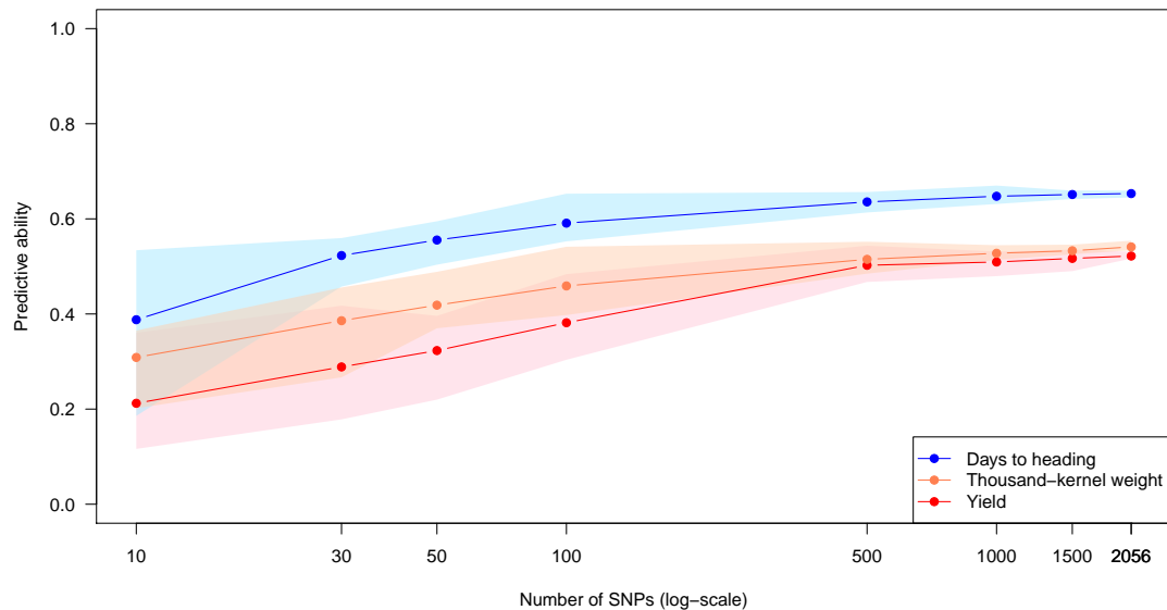
Figure S4 Predictive ability for marker subsets in the wheat data set. The predictive ability was estimated with fivefold cross-validation and 10 replications using RR-BLUP. Average predictive ability as a function of the number of randomly selected markers is visualized as a straight line for each trait. Shaded areas indicate the range of 10 different marker subsets.
