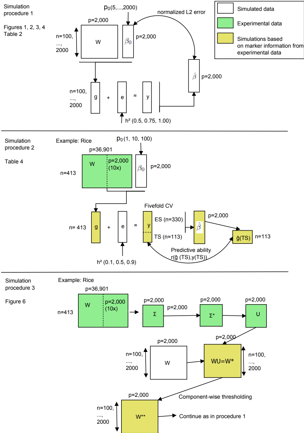
Figure S6 Overview of simulation procedures. For each simulation procedure, the resulting Tables and Figures are given. Procedures 2 and 3 were also conducted for the wheat and Arabidopsis data sets, respectively. Dashed lines indicate random sampling of individuals or markers.
