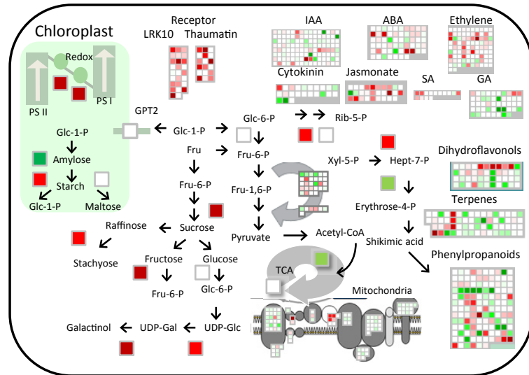
Figure S7. Overview of principal transcriptional changes induced by HLB (those in Fig. 2 along with those associated with hormone and secondary metabolism) induced by HLB in four tissues.
