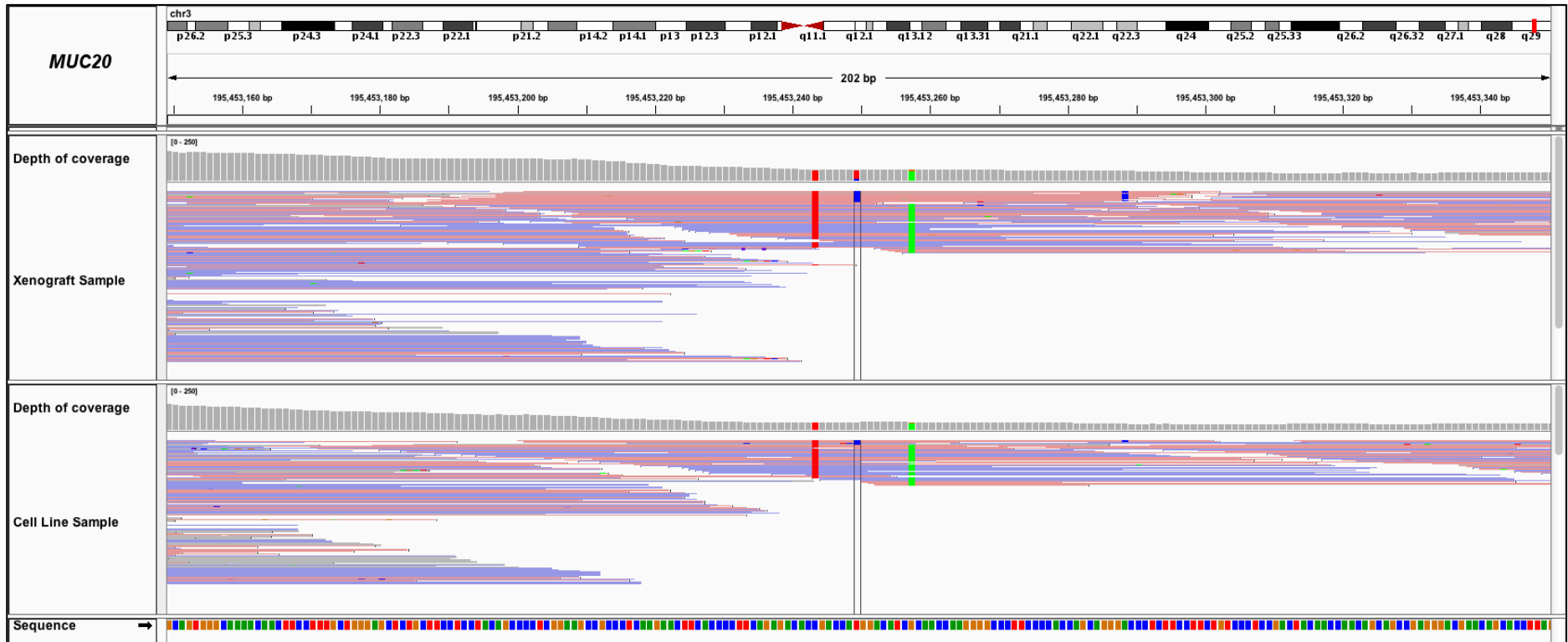
Figure S3. Analysis of xenograft-specific variants. Sequence depth of coverage and allele frequency comparisons between the xenograft and cell line samples. Both samples were aligned to the human reference genome hg19. Representative detected variants are shown for AQP7 (A), APEH (B), MUC17 (C) and MUC20 (D) genes. Genomic locations for the variants shown are described in supplementary Table 4 A. Variants position is highlighted by black parallel bars. Nucleotide residues are shown in red (thymine), blue (cytosine), green (adenine) and yellow (guanine). Heterozygous variants are indicated in the depth of coverage track and show both reference and alternative alleles. Forward and reverse sequencing reads are shown in pink and blue respectively. Sequence base mismatches are highlighted with its corresponding nucleotide color.
