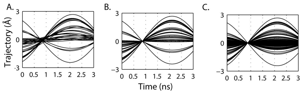
Figure S4. Transformation of reconstructed trajectories to reconstructed in-phase trajectories using PCA. (A) Reconstructed trajectories of three-Cartesian components of WPD loop C_{\alpha} atoms. (B) In-phase components obtained by employing PCA on the trajectories shown in (A). (C) In-phase components obtained by employing PCA on the reconstructed trajectories of C_{\alpha} atoms between residues 2 to 278.
