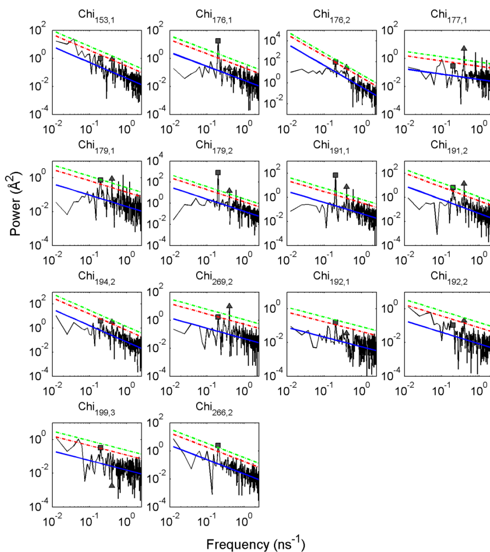
Figure S9. Power spectral density of various perturbed side-chain dihedral angles in the vicinity of WPD loop. Power component at 0.2 and 0.4 \text{ns}^{-1} are denoted by a square and a triangle, respectively.
