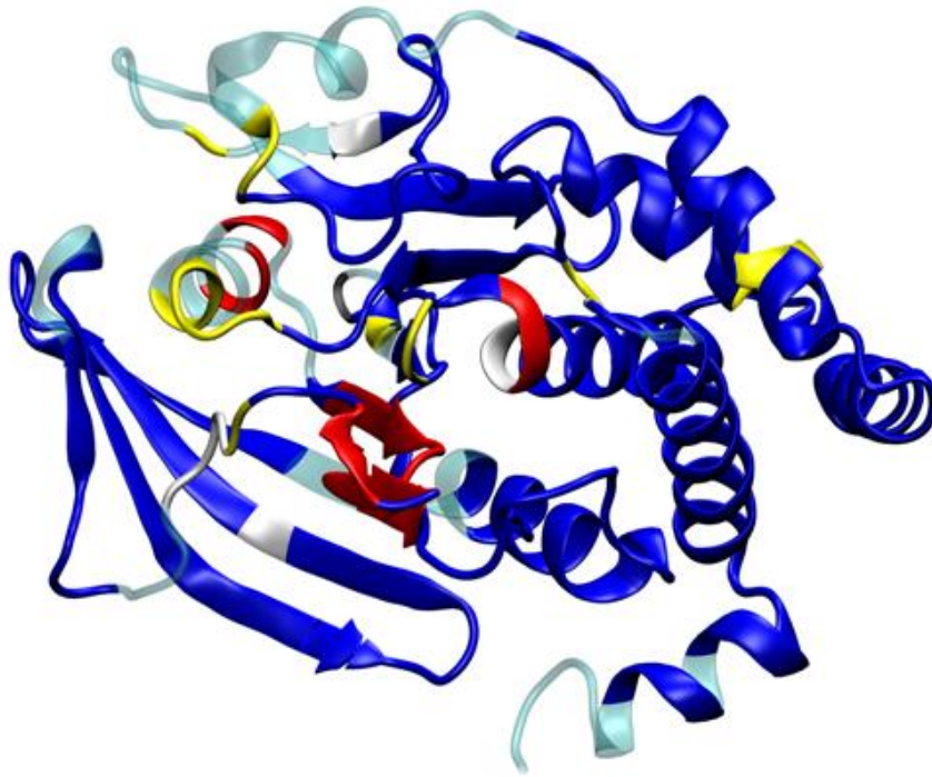
Figure S12. Classification of the residues with respect to their frequency responses. Blue and red colored residues have monotonic decreasing and monotonic increasing frequency responses, respectively. Concave functions may be fitted to the frequency responses of yellow residues, indicating an underdamped behavior. No definite trends in Bode plots of white residues have been observed (see Table S5). Transparent regions represent C_{\alpha} atoms not being perturbed by the TMD potential.
