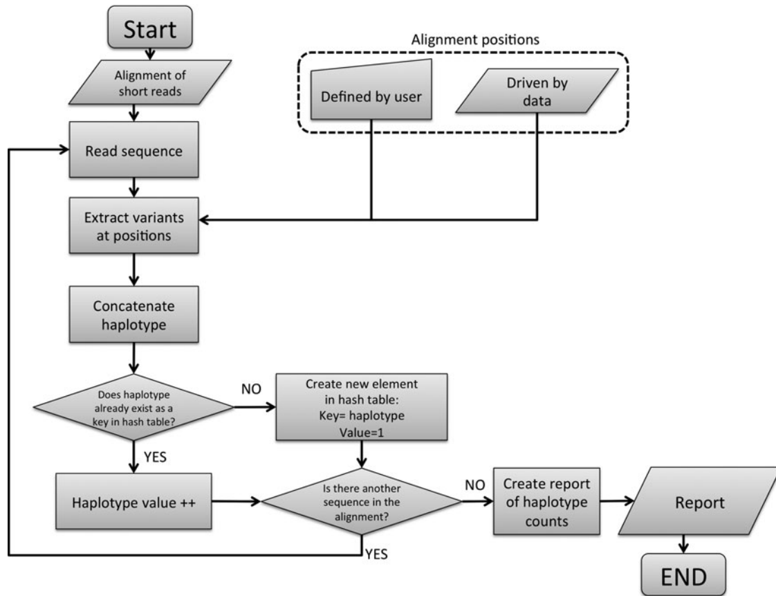
SUPPLEMENTARY FIG. S1. Flow chart of the algorithm implemented in DeepHaplo for the computation of haplotypes.
