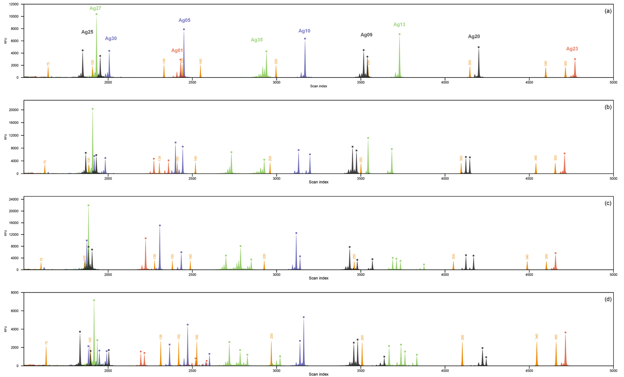
Supporting Figure S1: Example of fluorescent electrophoretic profiles for diploid (a, b) and tetraploid (c, d) A. glutinosa individuals genotyped at 12 microsatellite markers described in Lepais & Bacles (2011). Sized alleles are annotated with squares; size standard peak sizes are indicated above each corresponding peak. Locus names are shown in (a). Note Ag14 is missing in these four individuals probably due to presence of null alleles
