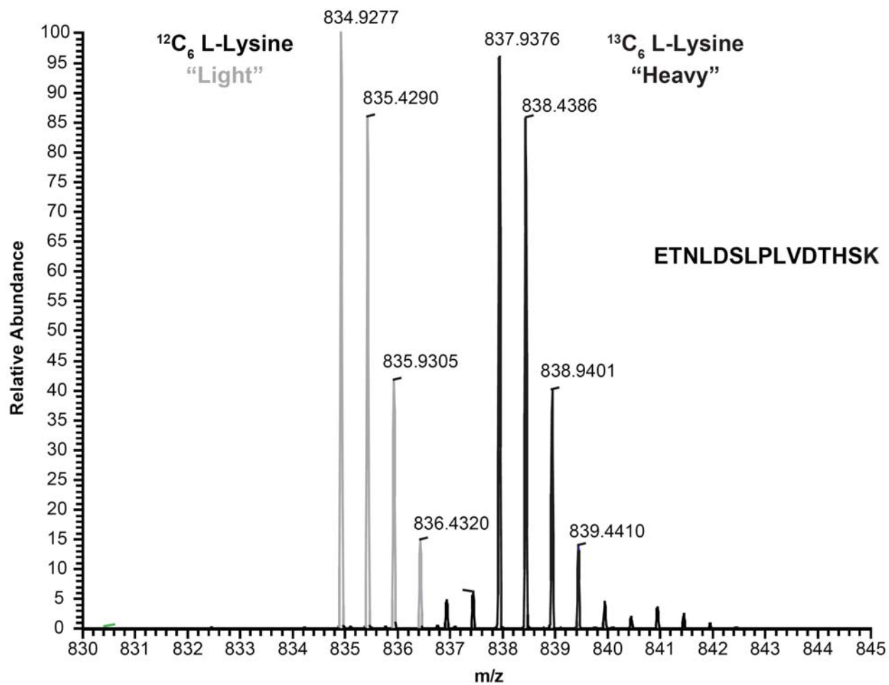
Supplementary Figure 1. Metabolic label incorporation. SILAC peak pairs for a double charged tryptic peptide from vimentin in a 1:1 mix of light and heavy samples. The mass difference between the light and heavy peptide is 6 Da.
