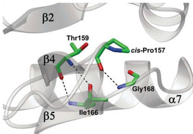
SUPPLEMENTARY FIG. S1. Hydrogen bond stabilization of the \beta 5 - \alpha 7 loop of ScsC protein of S. Typhimurium (StScsC). Hydrogen bonds between Ile 166 (O and NH) and Thr 159 (NH and O) and Gly 168 (NH) and cis-Pro 157 are shown as dashed lines.
