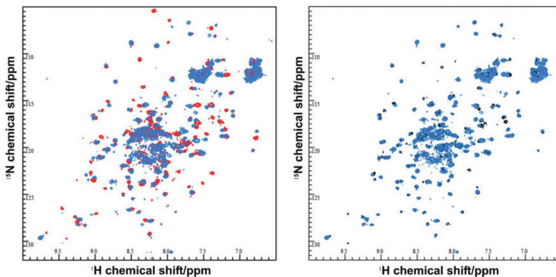
SUPPLEMENTARY FIG. S5. ^{15}\text{N} - ^1\text{H} HSQC spectra of fully oxidized and fully reduced StScsC. The spectra in blue on both panels are the fully reduced sample (treated with 5 mM DTT). Spectra in red and black are taken from the reduced glutathione/oxidized glutathione titration, and are fully oxidized and fully reduced, respectively. The peaks selected to calculate the reduction potential overlay with the fully reduced DTT sample.
