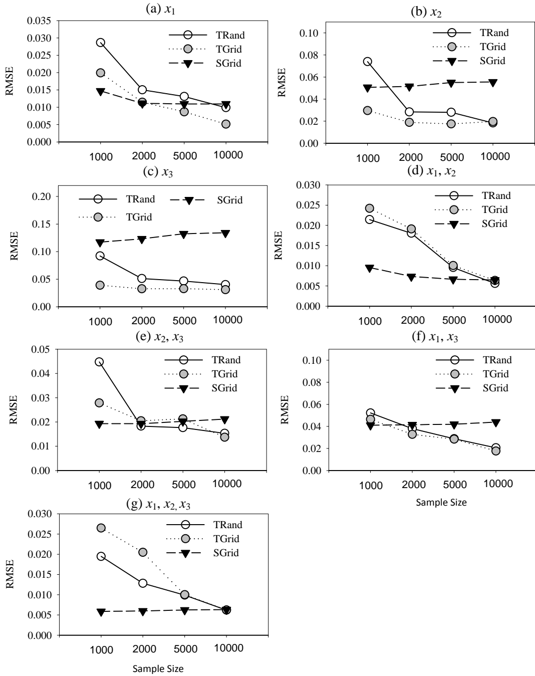
Figure S1 Comparison of different sampling methods (SGrid = search-curve based sampling using the auxiliary variable s ; TRand = simple random sampling in \theta -space; TGrid = random balance design sampling in the \theta -space) for root mean square error (RMSE) with different sample sizes (1000; 2000; 5000; and 10,000).
