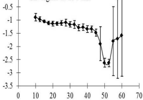
CD signal at 291 nm
