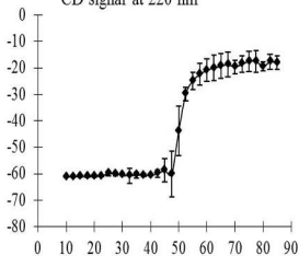
CD signal at 220 nm
