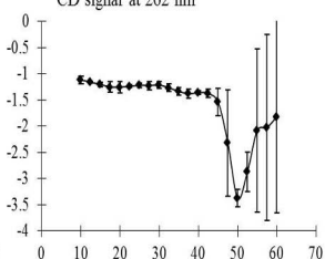
CD signal at 262 nm
