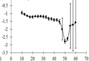
CD signal at 284 nm
