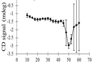
CD signal at 269 nm
