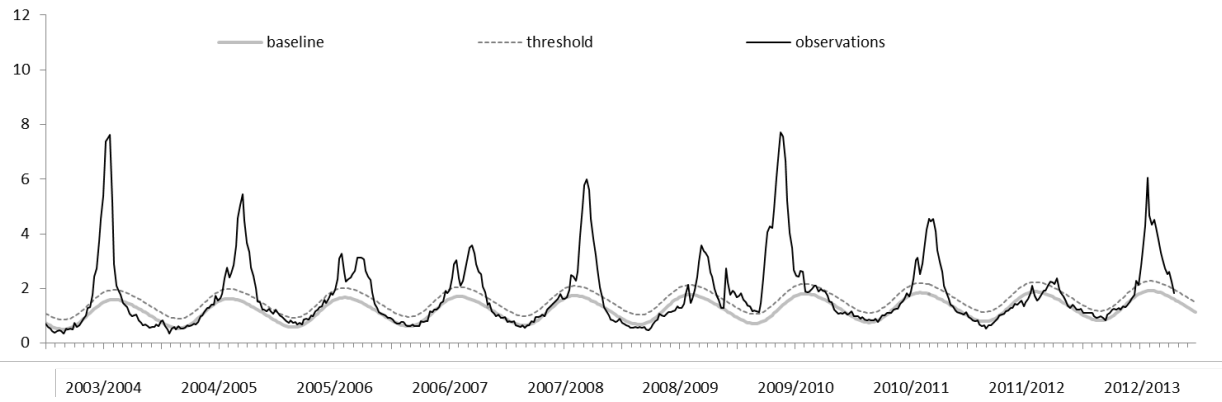
Figure S1 – National level influenza season observed and model baseline data, 2003-2013
