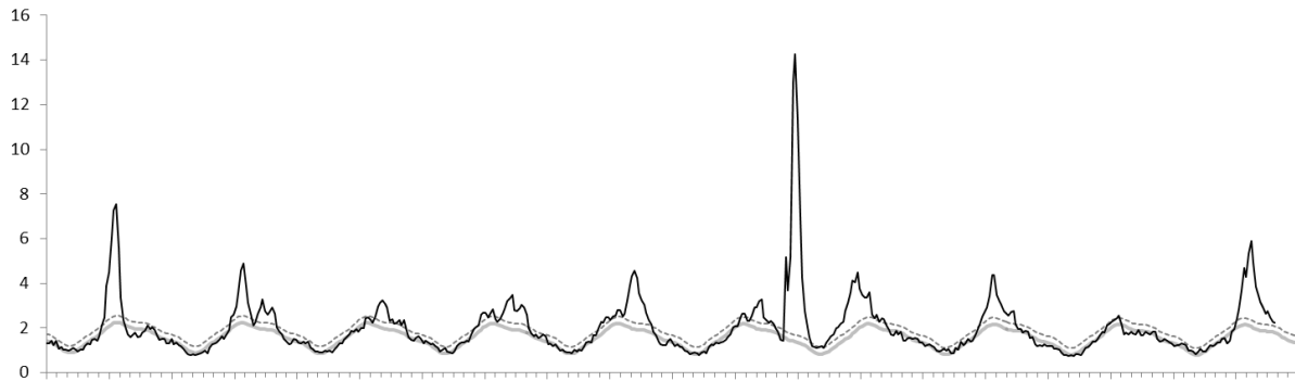
Figure S5 – New York influenza season observed and model baseline data, 2003-2013
