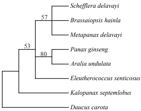
rps15-ycf1
