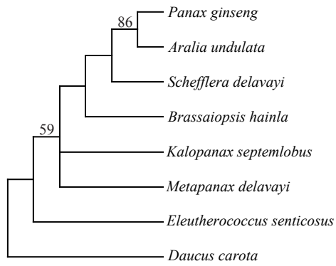
ndhF-rpl32
