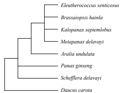
ndhG-ndhI
