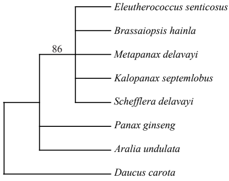
trnE(UUC)-trnT(GGU)
