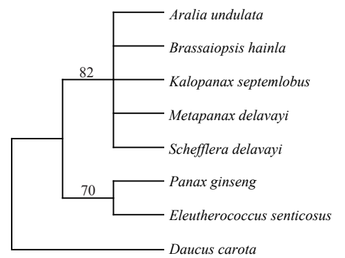
petB-intron
