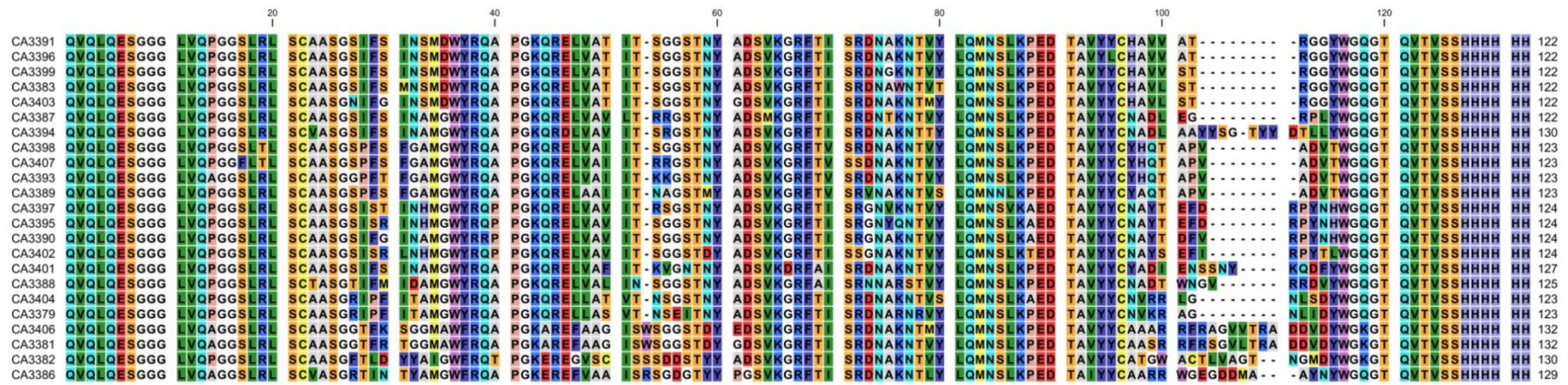
Supplementary Fig. S1. Sequence alignment of all 23 selected T2 specific binders. Corresponding CA-numbering for each nanobody can be found in Table 1.
