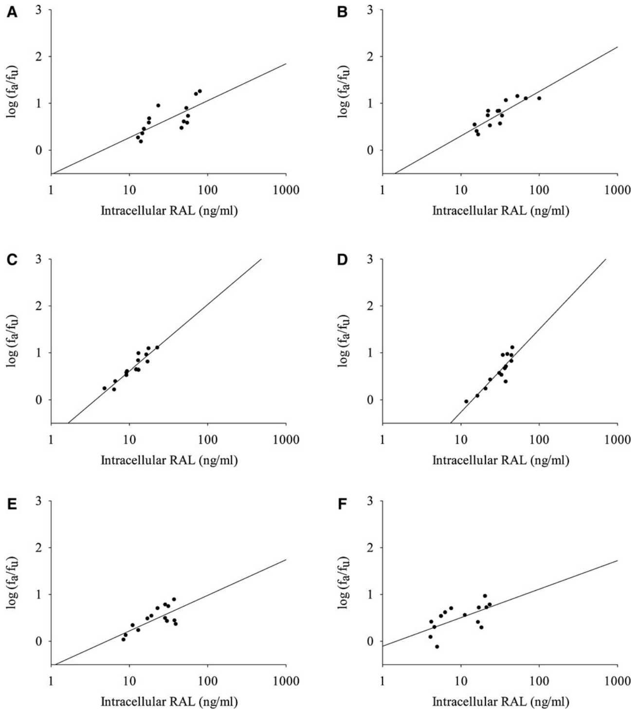
SUPPLEMENTARY FIG. S2. The impact of intracellular RAL on antiviral effect. The intracellular ARV concentrations and relative impact on antiviral effect were assessed using a median-effect model. (A–F) The intracellular dose-response relationship for six individual subjects CD4 + T cells following dosing with RAL. Response is measured as the \log_{10} of the fraction of virus affected by drug divided by the fraction of virus unaffected by drug ( f_a/f_u ).
