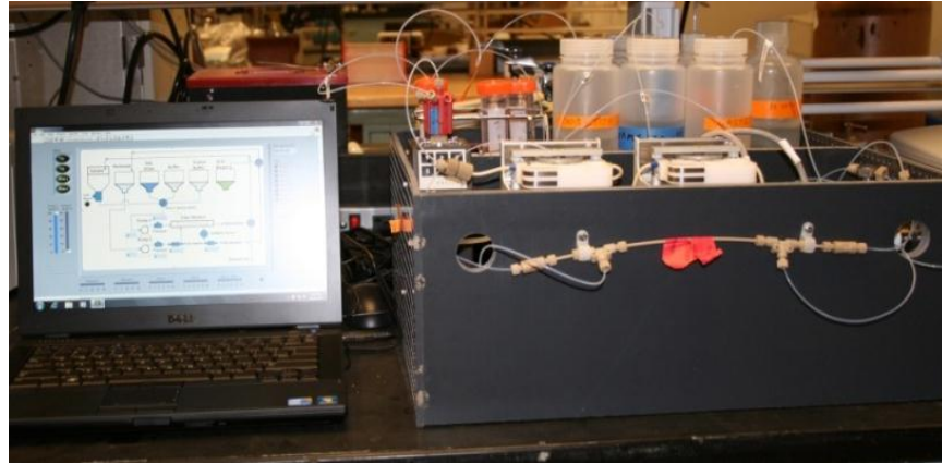
FIG S2 The Cell Concentration Instrument and the control interface in a laboratory PC
