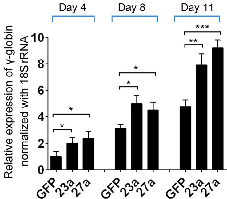
FIG. S3 The expression of \gamma -globin gene normalized with 18S rRNA in lentivirus-infected human CD34 + HPCs after Epo induction for 4, 8 and 11 days.
