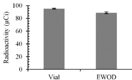
Supplementary Fig. 2 10 \mu\text{L} of an ^{18}\text{F} solution was pipetted into 5 source vials and 5 EWOD chips. Plotted is the average decay corrected radioactivity from the vials and EWOD chips. Error bars represent standard error of the mean. On average, the vial gives an activity measurement 6.8% greater than the EWOD chip.
