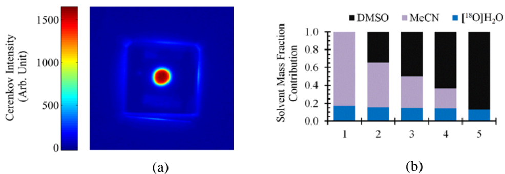
Supplementary Fig. 1 (a) Sample Cerenkov image of a \sim 5 \mu\text{L} mixed solvent droplet sandwiched between two Teflon-coated glass plates. (b) Solvent mass fraction contributions for each of the five mixtures measured.
