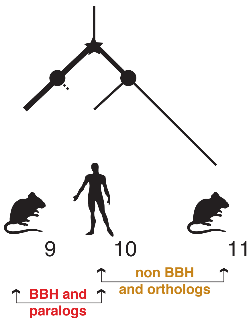
d) strong departure from molecular clock
