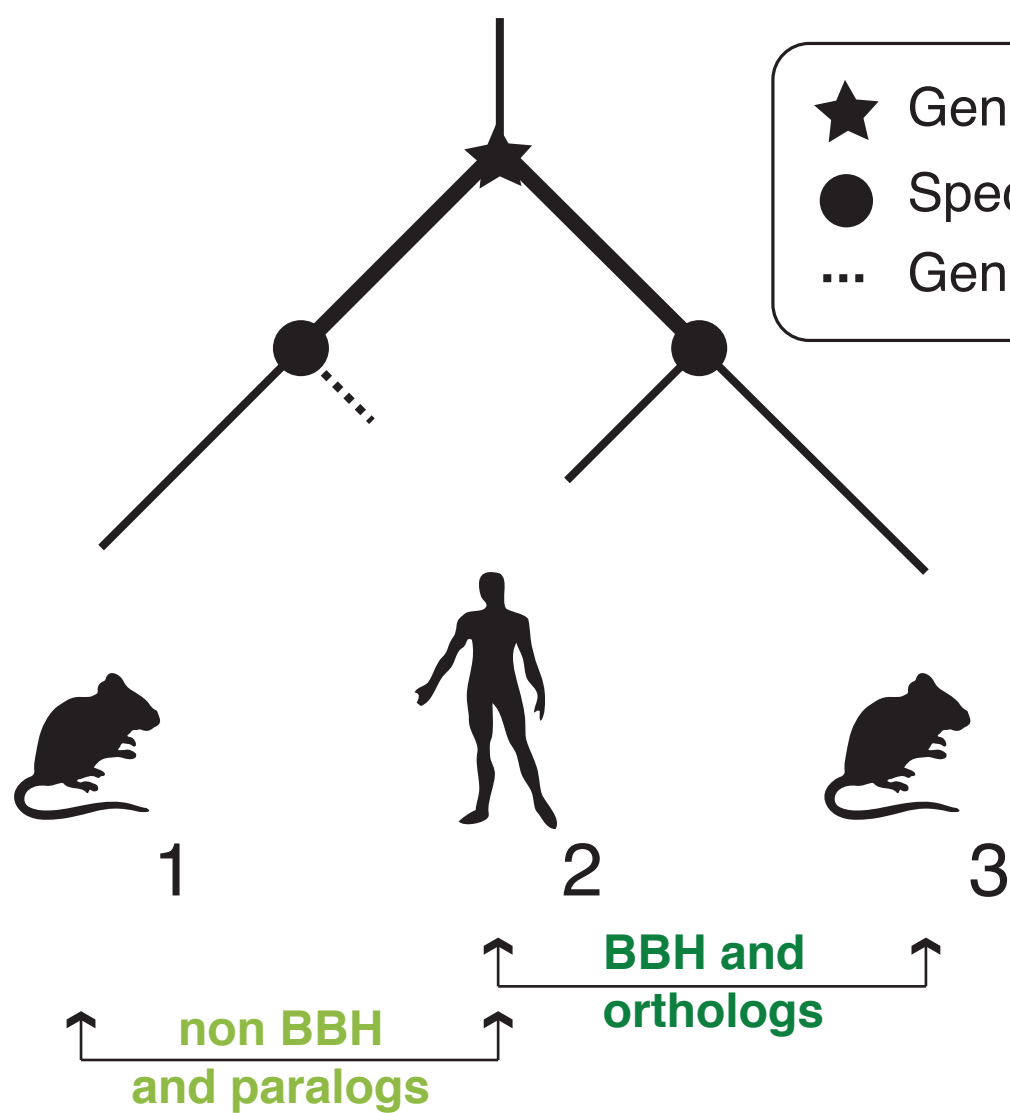
a) ancestral duplication
