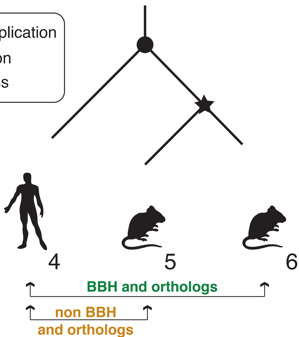
b) lineage-specific duplication
