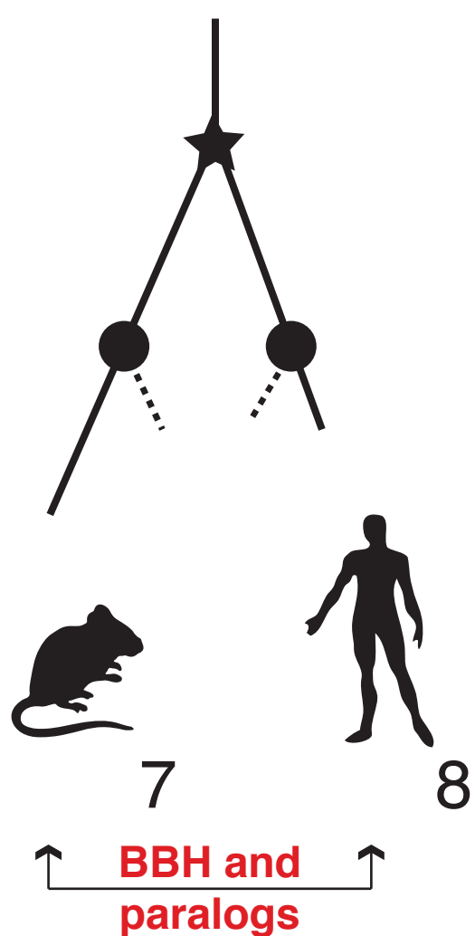
c) differential gene losses
