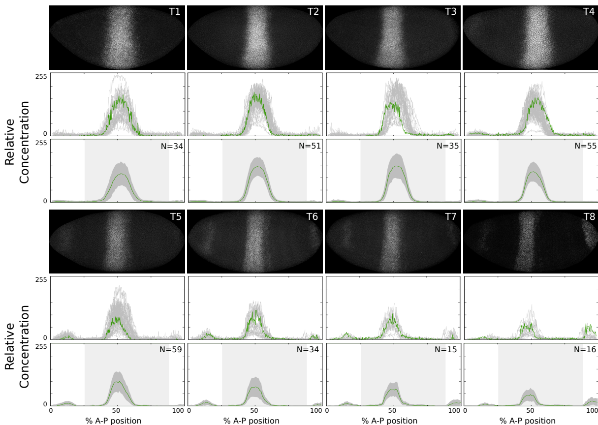
Figure S1. Quantification of Kr mRNA Data. Each panel represents a time class (T1–T8) in C14A showing an example embryo image (top), un-registered expression profiles (middle), and integrated expression patterns (bottom, with standard deviations shown as dark grey background). Embryo images show lateral views: anterior is to the left, dorsal up. Graphs plot relative mRNA concentration against A–P Position (in %, where 0% is the anterior pole). Expression profiles consider only the central 10% strip along the dorso-ventral axis. Green profiles in middle panels were extracted from embryos shown in images above. Lightly shaded background in lower panels represents the region of the embryo considered in our models. See Materials and Methods for details on data processing.
