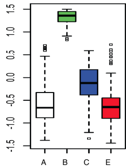
cluster V (198)
