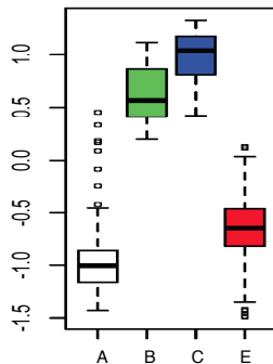
cluster III (157)
