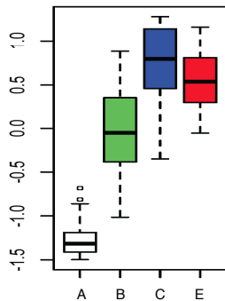
cluster VIII (86)
