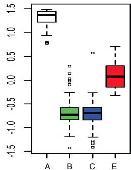
cluster I (102)
