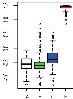
cluster VII (216)
