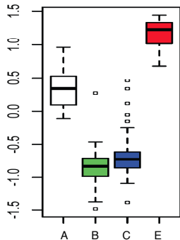
cluster II (71)
