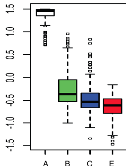
cluster IV (163)
