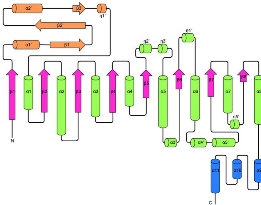
Figure S2 Topology of the overall structural fold of CmIDCase. The (\beta/\alpha)_8 barrel domain is shown with \alpha -helices in green and \beta -strands in magenta. The insertion domain is colored in orange, and the C-terminal three \alpha -helices in blue.
