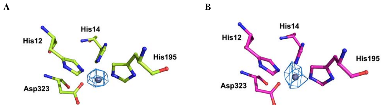
Figure S5 Anomalous dispersion analyses of CmIDCase and MaIDCase. (A) The anomalous difference Fourier map (5.0 \sigma contour level) of the bound Zn 2+ in the apo CmIDCase structure. (B) The anomalous difference Fourier map (5.0 \sigma contour level) of the bound Zn 2+ in the apo MaIDCase structure.
