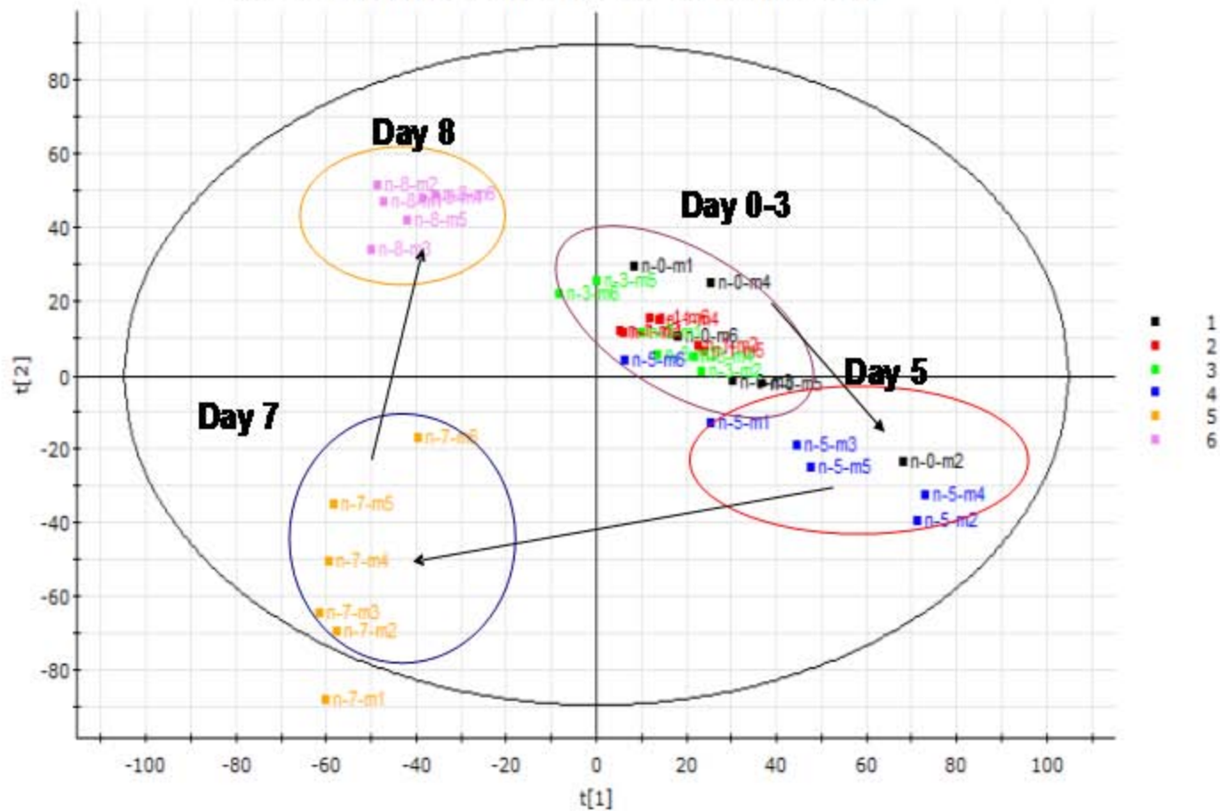
Scores Comp[1] vs. Comp[2] colored by Sample Group
