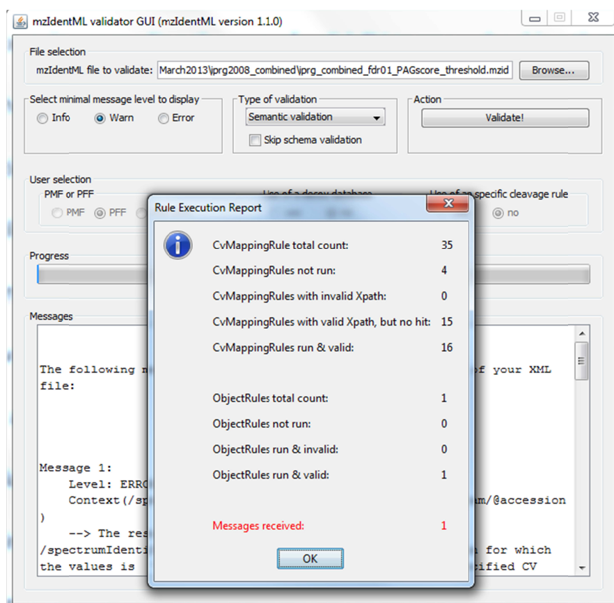
S. Figure 2. A screenshot of the mzidValidator showing the summary output and the detailed output behind with validation errors and pointers to the positions in the file causing errors.
