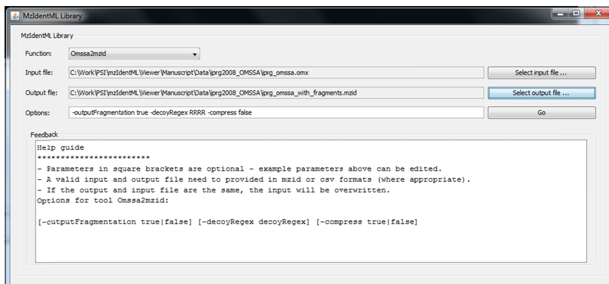
S. Figure 1. A screenshot of the basic graphical interface for calling the mzidLibrary.
