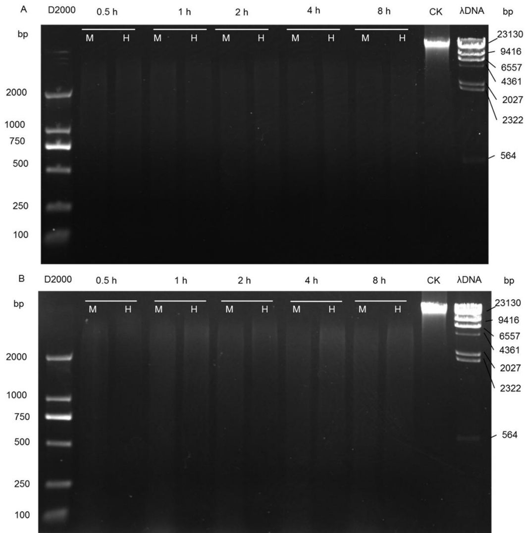
Fig S1 Restriction digestion efficiency identification. (A) II-32B; (B) Huhan-3. M represent EcoR I /Msp I lane, H represent EcoR I /Hpa II lane, CK was negative control.
