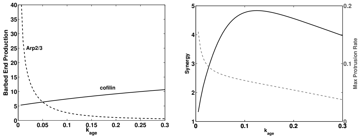
Figure S4: Effect of the F-actin aging rate k_{age} on barbed end production and synergy. Left : Barbed end production ( B_{prod} ) in the presence of cofilin only (solid curve) and Arp2/3 only (dashed curve). Right : Synergy (black solid curve, left axis) and barbed end production (grey dashed curve, right axis) in the presence of both cofilin and Arp2/3. ( J_C = 1.6 \mu\text{M}\cdot\mu\text{m/s} , A_{edge} = 44 \mu\text{M} , as in Fig. 3), simultaneous cofilin and Arp2/3 stimulation ( 0 < t < 10\text{s} ). Other parameters as in Table S1.
