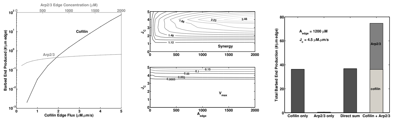
Figure S7: Barbed end production and synergy with highly localized Arp2/3 ( \epsilon = 10^{-6} \mu\text{m/s} ). Left: Barbed end production curve when cofilin and Arp2/3 act alone. Middle: Synergy and maximum protrusion rate for varying stimulation amplitude. Right: Comparison of total barbed end production using stimulation size of A_{edge} = 1200 and J_c = 4.5 ( S=2.03 ).
