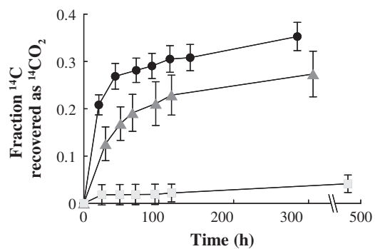
SUPPLEMENTARY FIG. S2. Effect of ammonium nitrate concentration on mineralization of ^{14}\text{C} -anthracene in batch incubations containing bioreactor-treated slurry. Other notation as in Supplementary Fig. S1.
