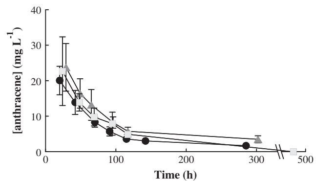
SUPPLEMENTARY FIG. S3. Effect of ammonium nitrate concentration on disappearance of unlabeled anthracene in batch incubations containing bioreactor-treated slurry. Symbols and error bars represent the mean and range of duplicate incubations. Other notation as in Supplementary Fig. S1.
