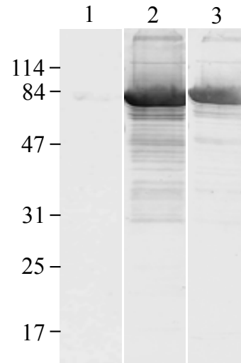
FIG S2. Detection of anti-CbpB IgG antibodies in convalescent-phase sera from naturally E. rhusiopathiae -infected pigs. Lanes: 1, control serum from a non-infected pig; 2, convalescent pig serum with an IgG growth-agglutination (GA) titer of x256; 3, convalescent pig serum with an IgG GA titer of x64. The sera were diluted 1:1,000 in PBS, and the bound antibodies were detected with horseradish peroxidase-conjugated rabbit anti-pig IgG (Zymed Laboratories). The positions of the protein molecular mass standards (kDa) are shown to the left.
