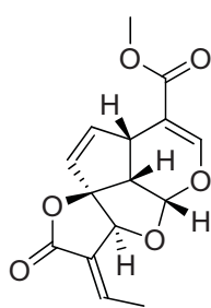
(II) Plumericin
