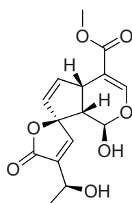
(III) Plumieridin
