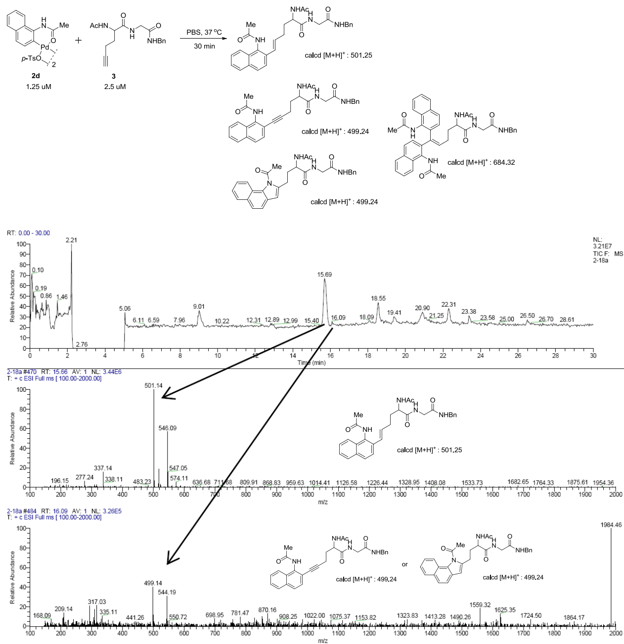
Figure S4. LC-MS analysis of the reaction of palladacycle 2d with N -acylated HPG-dipeptide 3 . 5
