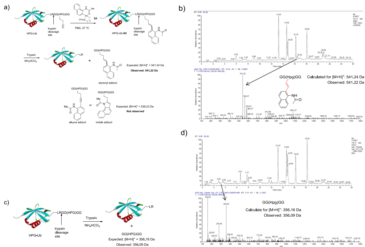
Figure S1. Trypsin digestion and LC-MS analysis of the HPG-Ub- 2d cross-coupled product: a) Reaction scheme; b) LC-MS analysis of the tryptic reaction mixture showing the identification of the styrenyl adduct; c) Trypsin digestion of the unlabelled HPG-Ub; d) LC-MS analysis of the tryptic HPG-Ub mixture showing the identification of the the GG(Hpg)GG fragment.
