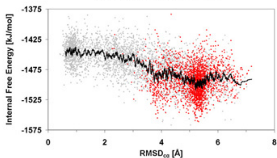
UA Backbone Electrostatics
