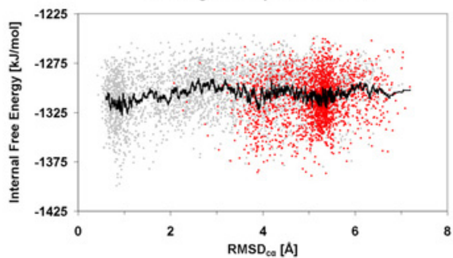
UA Charged Group Electrostatics
