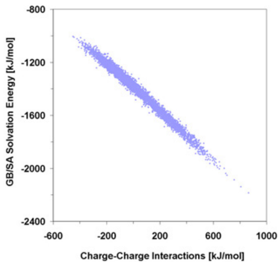
Electrostatic Interactions vs Solvation
