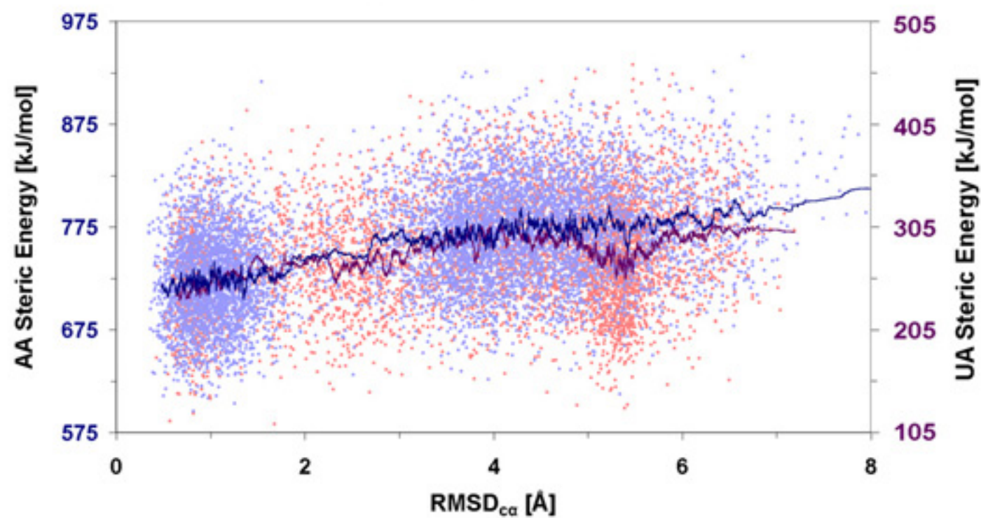
UA versus AA Sterics
