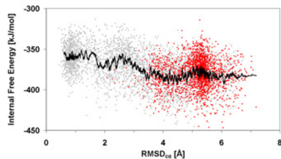
UA Neutral Side-Chain Electrostatics
