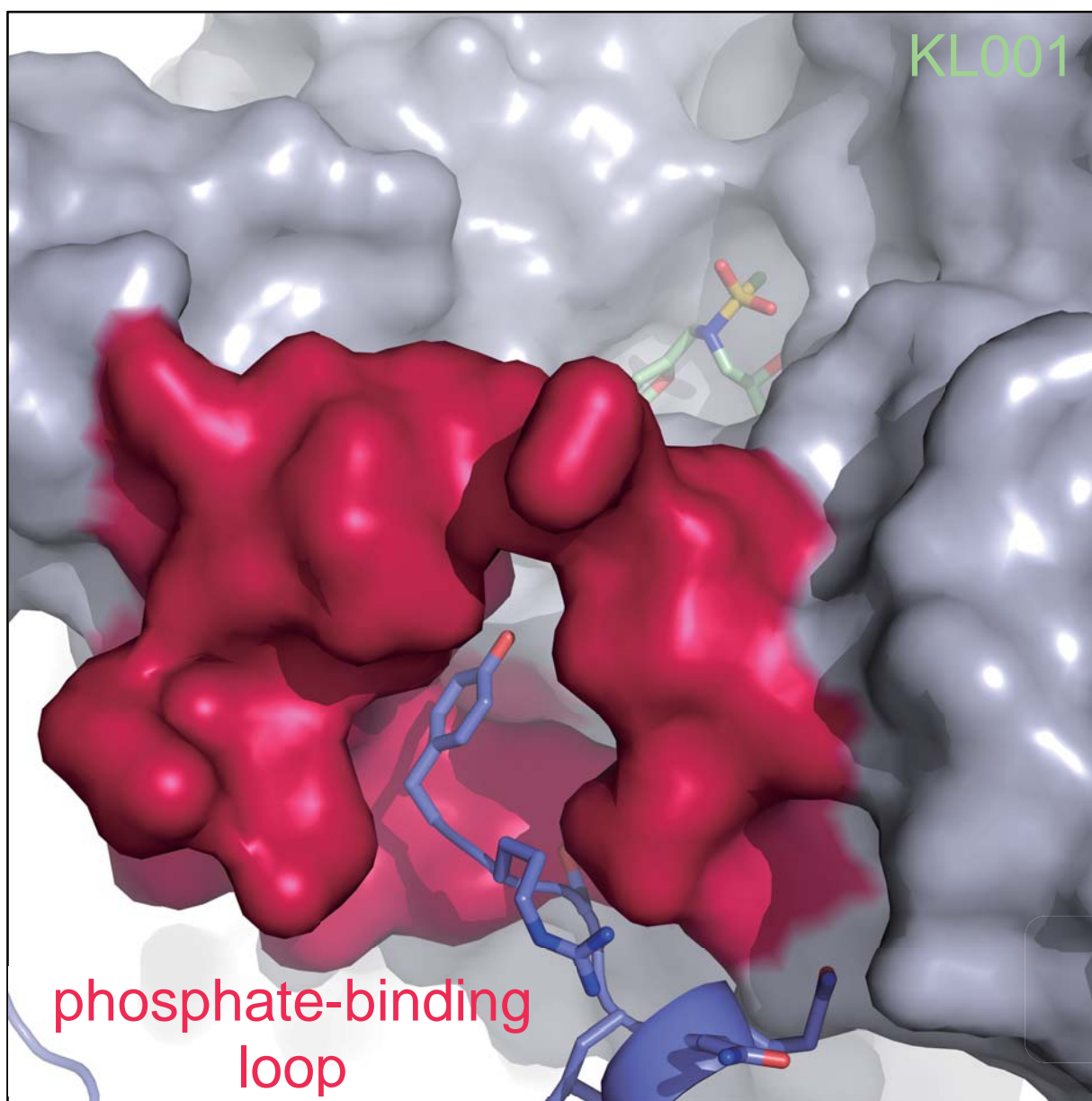
Figure S4. Stabilization of mCRY2 phosphate-binding loop by crystal packing. A close up view of the interaction between the phosphate-binding loop and the C-terminal Tyr residue (blue) of a nearby molecule in the crystal. KL001 (green) is at the opposite end of the FAD-binding pocket to the phosphate-binding loop.
