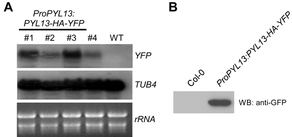
Supplementary information, Figure S3 Expression of PYL13-3HA-YFP in ProPYL13: PYL13-HA-YFP transgenic lines. (A) Analysis of YFP expression in ProPYL13: PYL13-HA-YFP lines using Northern blotting. Ethidium bromide stained rRNA bands are shown as the loading control. (B) Detection of the PYL13-HA-YFP protein in a sample purified from floral organs of ProPYL13: PYL13-HA-YFP -expressing lines without external ABA using anti-GFP-agarose. PYL13-HA-YFP protein was detected with anti-GFP mouse antibodies (Roche).
