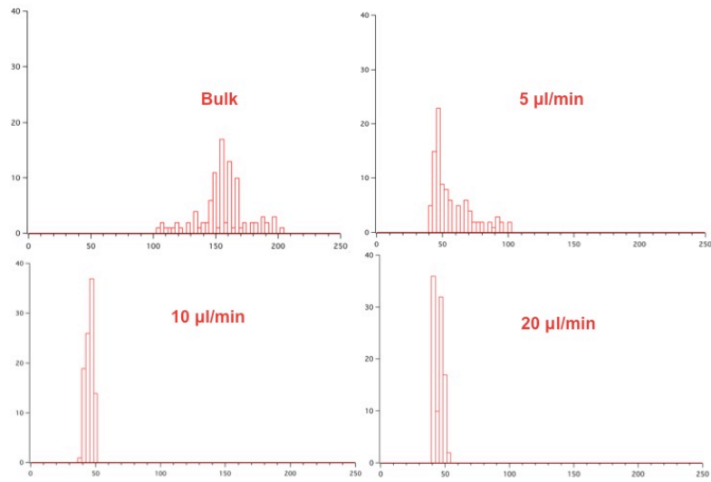
Figure S3. AFM size distributions of nanocomplexes produced by bulk mixing and flow mixing at pDNA flow rates of 5, 10 and 20 \mu\text{L}/\text{min} .
