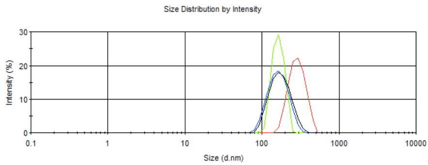
Figure S2. Size distributions by intensity of nanocomplexes produced by (red) bulk mixing and flow mixing at pDNA flow rates of (black) 5, (blue) 10 and (green) 20 \mu\text{L}/\text{min} .
