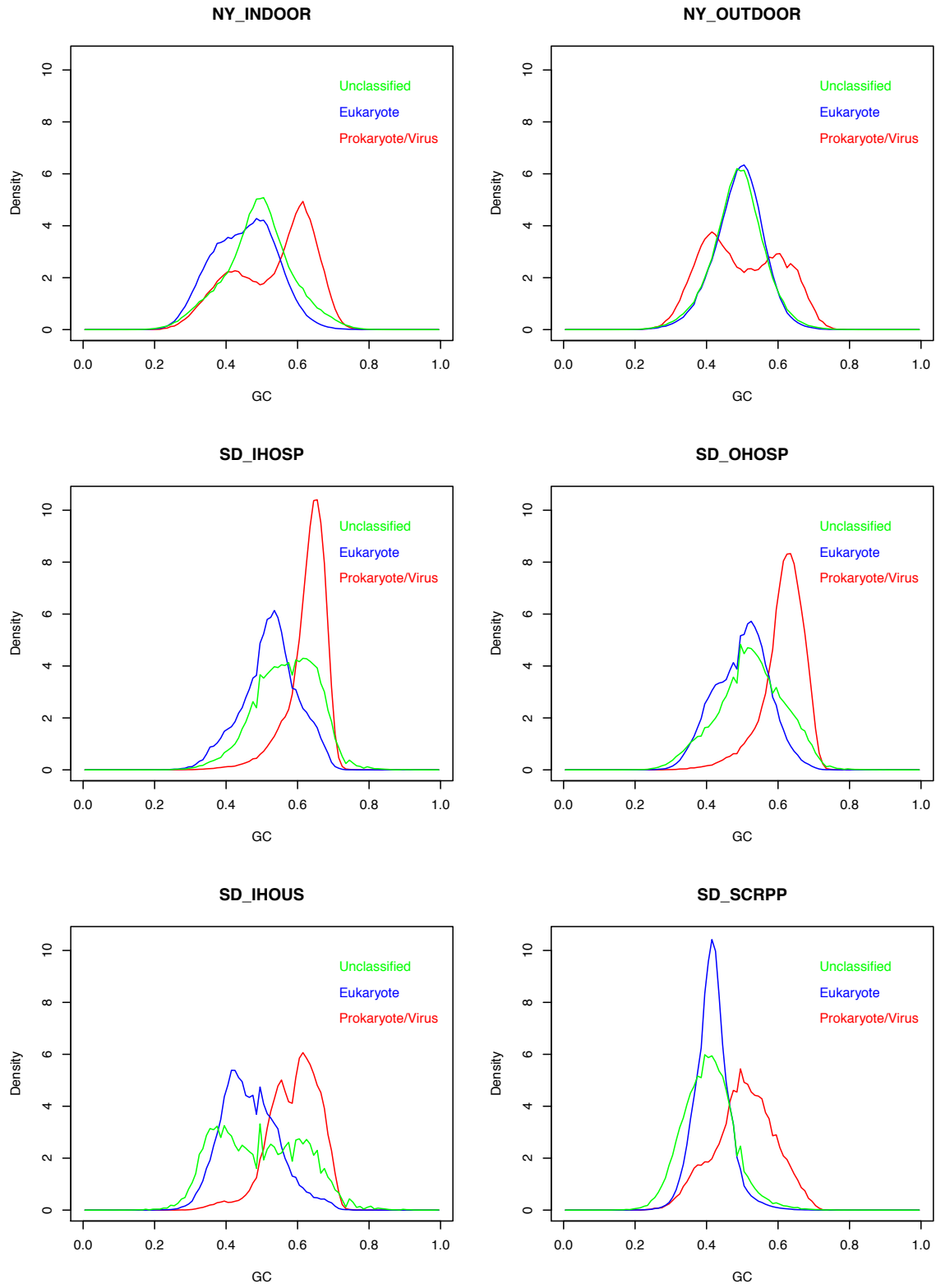
Figure S2: GC composition profile for the unclassified group (U), eukaryotic group (E), and prokaryotic/viral group (PV).
