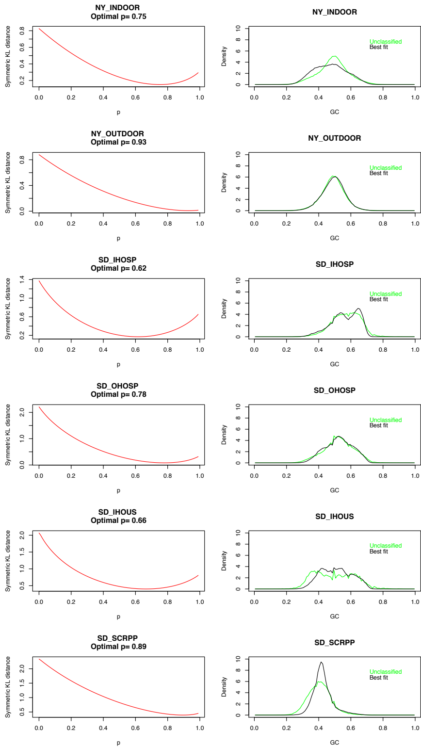
Figure S3: Best fit curves for the mixture modeling using the optimal value of p .
