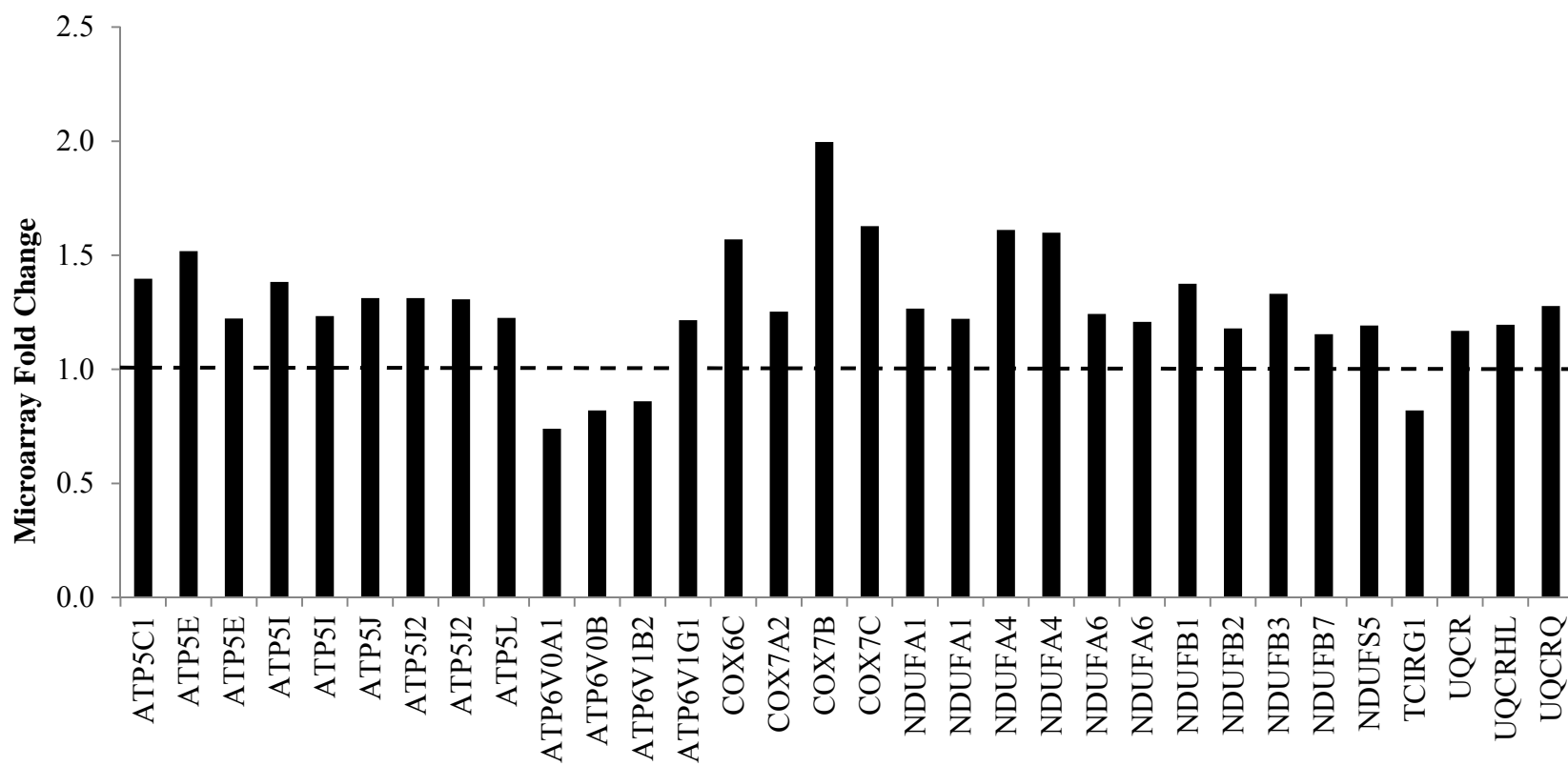
Figure S1 Oxidative phosphorylation genes with altered expression in individuals with metabolic syndrome. The dashed line indicates no change in gene expression. All probes were altered in expression \geq 1.2 fold and P < 0.05 (Benjamini corrected)
