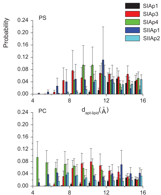
SUPPLEMENTARY FIG. S1. Probabilities of designed aptamers and lipid at a specific separation distance ( d ). The histograms plot probabilities of designed aptamers away from phosphatidylserine (PS) at d_{\text{apt-PS}} distance ( upper panel ) and away from phosphatidylcholine (PC) at d_{\text{apt-PC}} ( lower panel ) during 10-nanosecond simulations. Note that all probability points are calculated within every consecutive 1Å interval.
