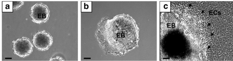
SUPPLEMENTARY FIG. S1. EB formation and EB coculture with HMECs. (a) EB day 3 in suspension. (b) EB day 6 cultured alone attached to a coverslip. (c) EB day 15 cocultured with HMECs (cell-cell interphase indicated by black arrows ). Scale bars = 100 \mu\text{m} . EBs, embryoid bodies; HMECs, human microvascular endothelial cells.
