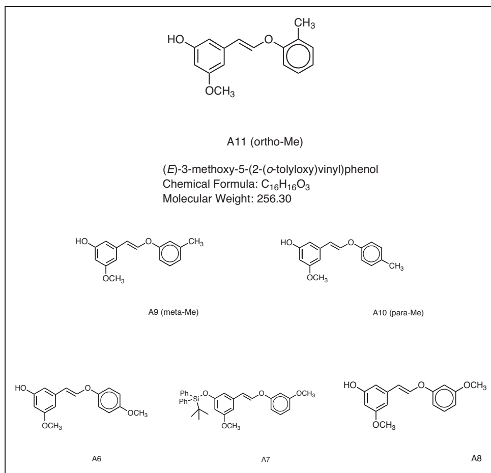
Supplementary Fig. S2. Chemical structure of the bioactive vinyl ether A11 and its analogs.
