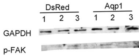
SUPPLEMENTARY FIG. S7. Western blot of p-FAK in Aqp1-MSCs and DsRed-MSCs. Total protein of Aqp1-MSCs and DsRed-MSCs was extracted and blotted with p-FAK (Y397) and GAPDH antibodies.
