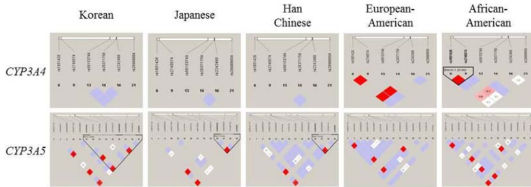
Supplemental Fig. 2. LD blocks of CYP3A4 (upper panel) and CYP3A5 (lower panel) with five ethnic groups which are comprised of Korean, Japanese, Han Chinese, European-American, and African-American. The LD structures were calculated using SNPs which showed frequencies in more than two populations.
