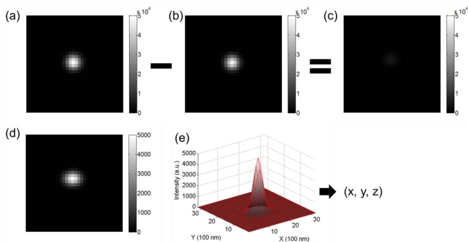
SI Figure 5. (a) Simulated image of 11 quantum dot: 11 are on; (b) Simulated image of the same 11 quantum dots in (a) but one of the quantum dot undergoes a transition from on to off: 10 are on while 1 is off; (c) Subtraction of (b) from (a) results in the PSF of the single quantum dot in the off state; (d) Same as (c) but the color-bar is rescaled; (e) Two-dimensional Gaussian fitting of (d) gives the position of the quantum dot.
