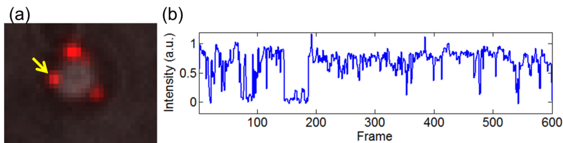
SI Figure 10. (a) Sample of quantum dots (red) on the surface of a bead (gray). (b) Intensity trace of the quantum dot, indicated by the yellow arrow in (a), showing two states.
