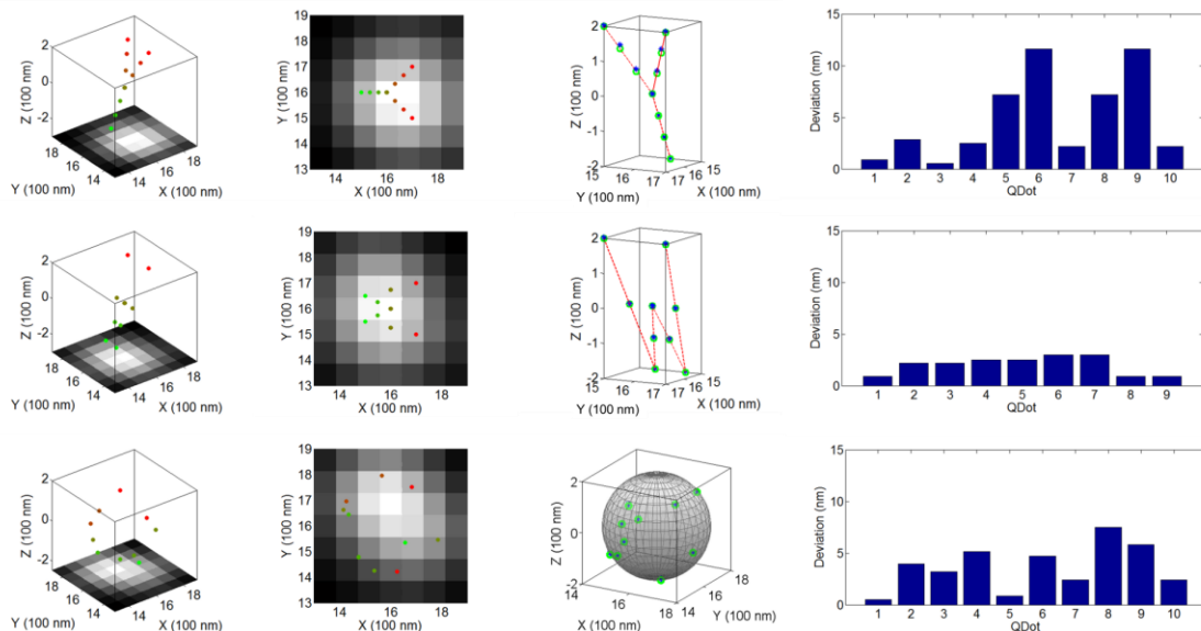
SI Figure 3. Three-dimensional images obtained by QDB3 from simulated movies of quantum dots with patterns of a letter Y (top), a letter W (middle) and a random spherical distribution (bottom) in the absence of noise.
