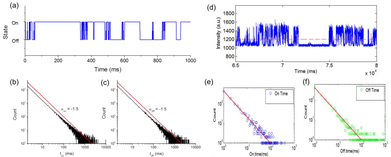
SI Figure 2. Blinking of simulated quantum dots and real quantum dots. (a) An example of the trace of a quantum dot used in simulated movies is shown. The probabilities of the on-time (b) and off-time (c) obey a power law: P(t) \propto t^{-\alpha} , where \alpha_{\text{on}} = -1.5 and \alpha_{\text{off}} = -1.5 (red lines with slopes of -1.5 are shown). (d) An example of the intensity trace of a real quantum dot used in the experiments (measured at temporal resolution of 1 ms). It is confirmed that the probabilities of the on-time (e) and off-time (f) follow power-laws.
