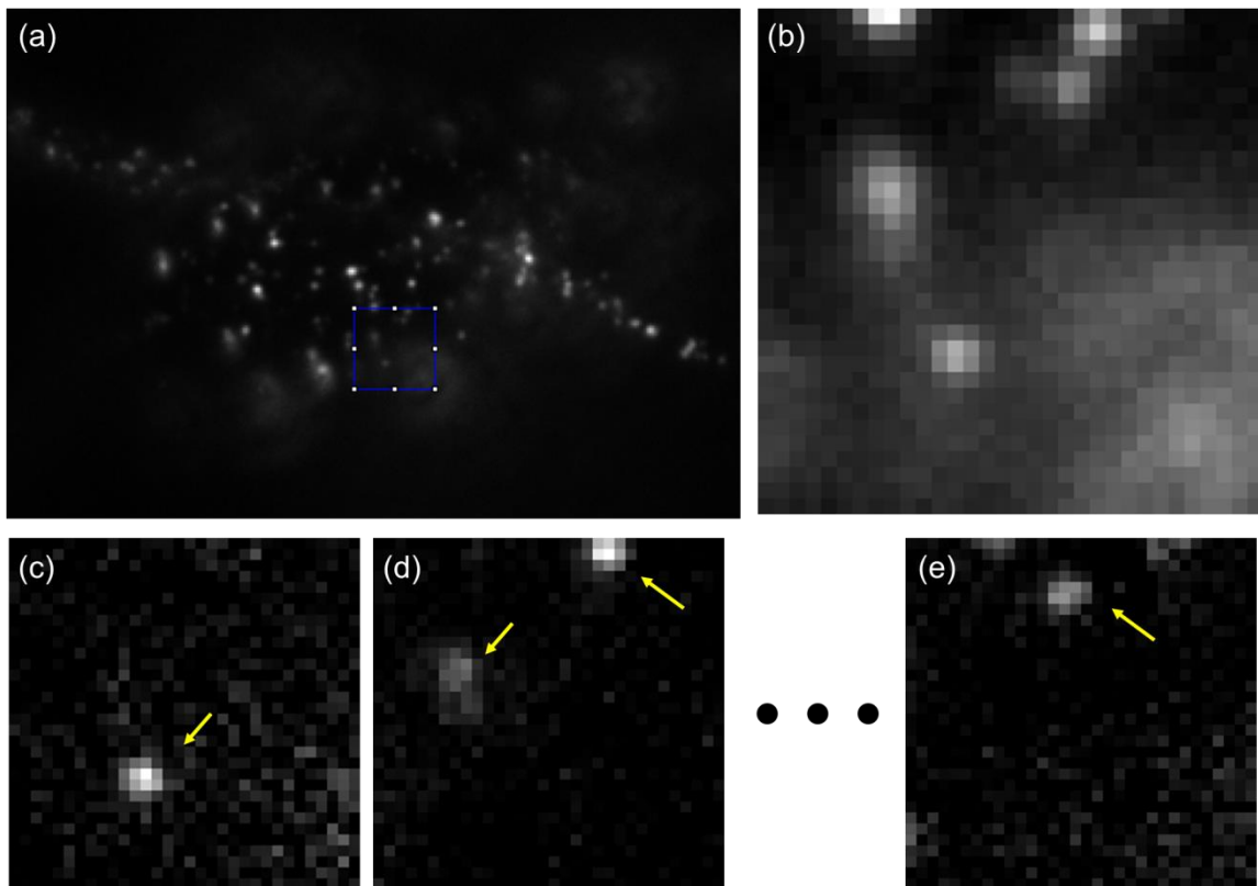
SI Figure 7. (a) Image from a breast cancer cell using normal fluorescent microscopy (from real data shown in Figure 7a); (b) Zoom-in of the rectangular region in (a); (c-e) A few frames from the intermediate movie show “ activated ” quantum dots.
