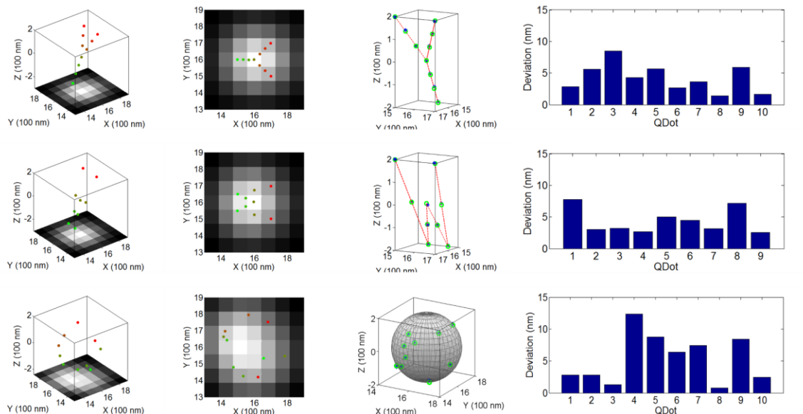
SI Figure 4. Three-dimensional images obtained by QDB3 from simulated movies of quantum dots with patterns of a letter Y (top), a letter W (middle) and a random spherical distribution (bottom) in the presence of Poisson noises.
