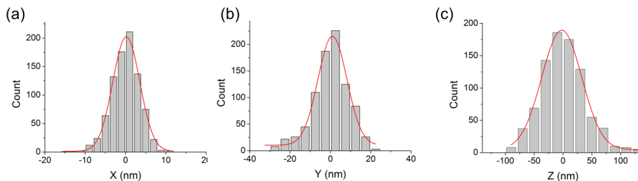
SI Figure 11. Histograms of the localization distribution in x, y, and z (from 5 quantum dots on surfaces of beads). The distributions were fitted to Gaussian functions, yielding standard deviations of \sigma_x = 3.3 \pm 0.1 nm, \sigma_y = 7.2 \pm 0.5 nm, and \sigma_z = 34.6 \pm 1.3 nm.
