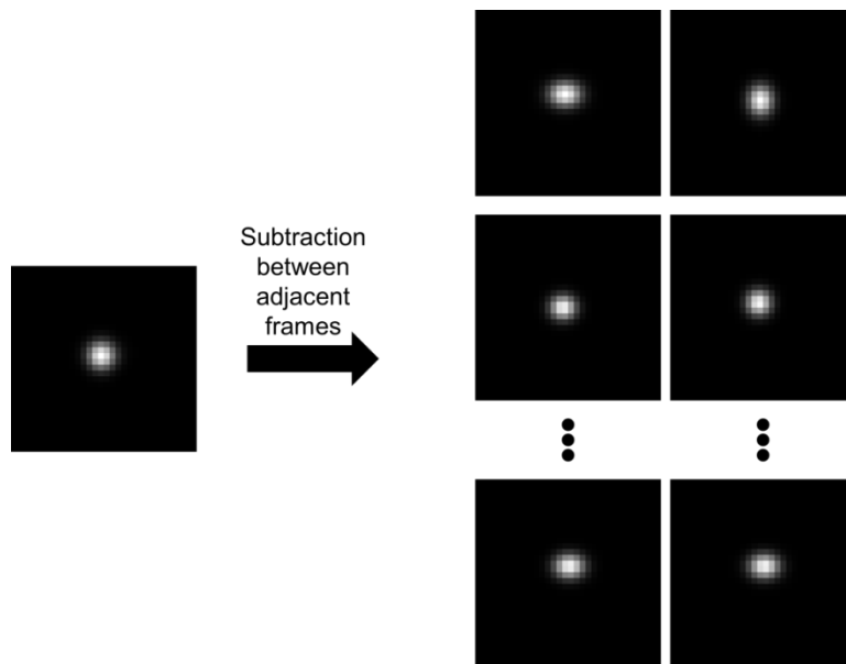
SI Figure 6. Repeating the process in SI Figure 5 on a movie (left) gives a series of intermediate images (right), consisting of an intermediate movie.
