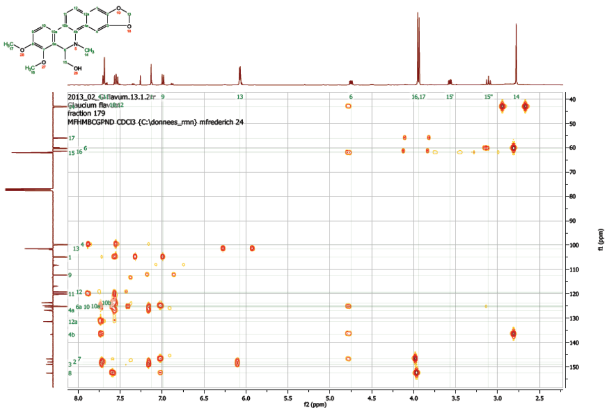
Figure S4. HMBC-NMR Spectroscopic data of compound 6 (500 MHz, \text{CDCl}_3 ).
