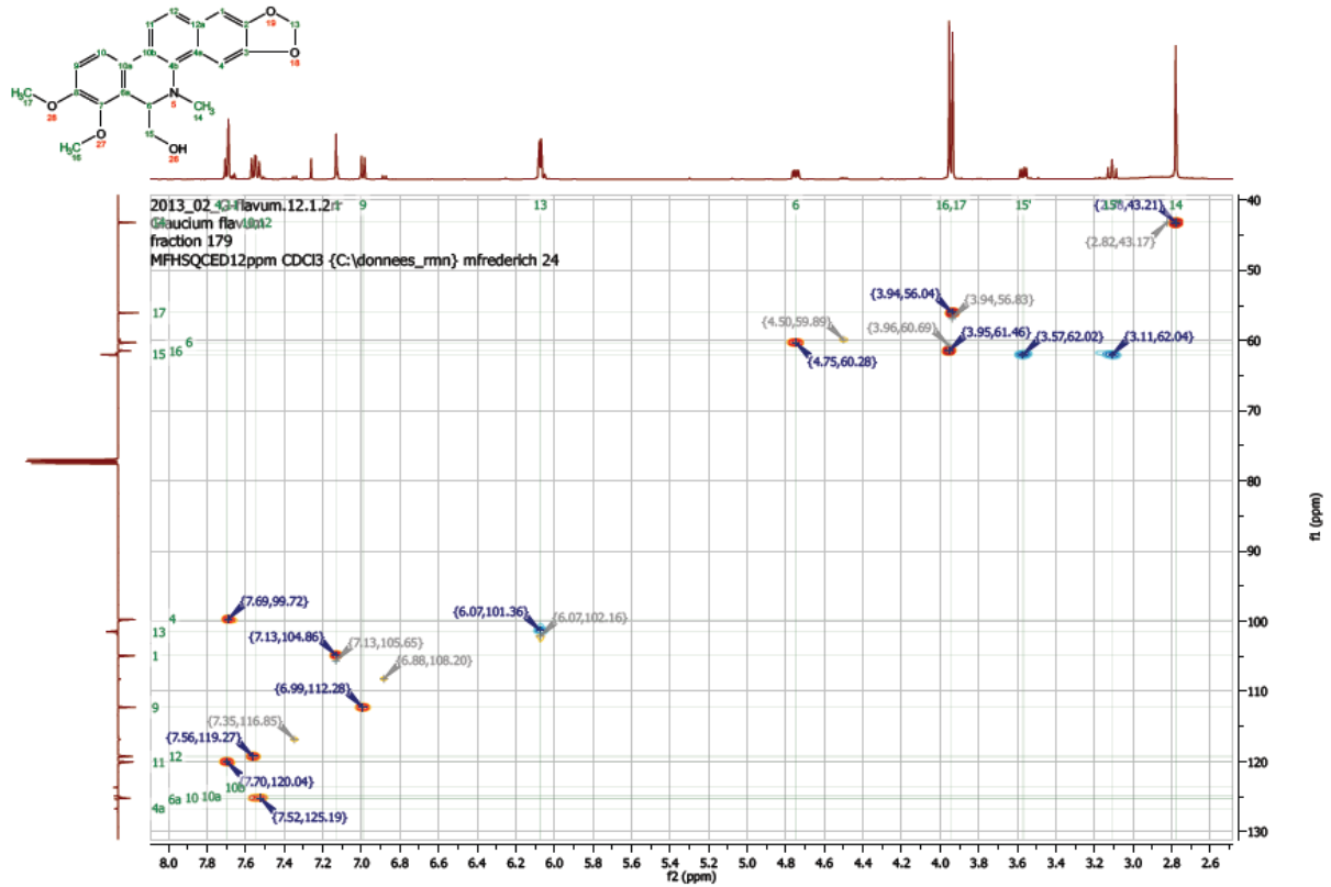
Figure S5. HSQC-NMR Spectroscopic data of compound 6 (500 MHz, CDCl 3 ).
